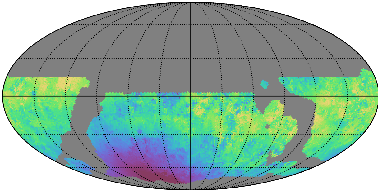
weather_cloudso6v3.4_10yrs WFD u band: Median moonDistance
