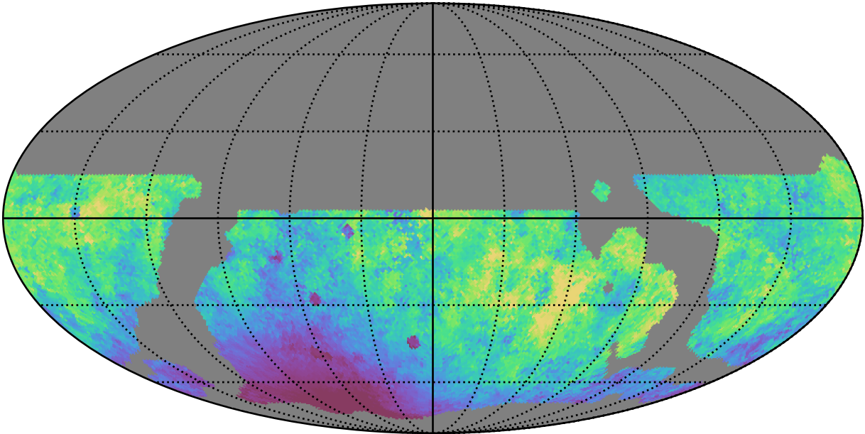
weather_cloudso6v3.4_10yrs WFD r band: Median moonDistance
