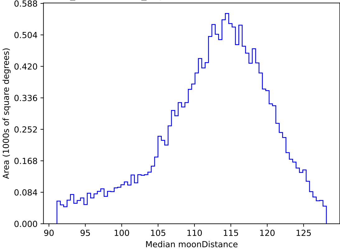
weather_cloudso6v3.4_10yrs WFD r band: Median moonDistance
