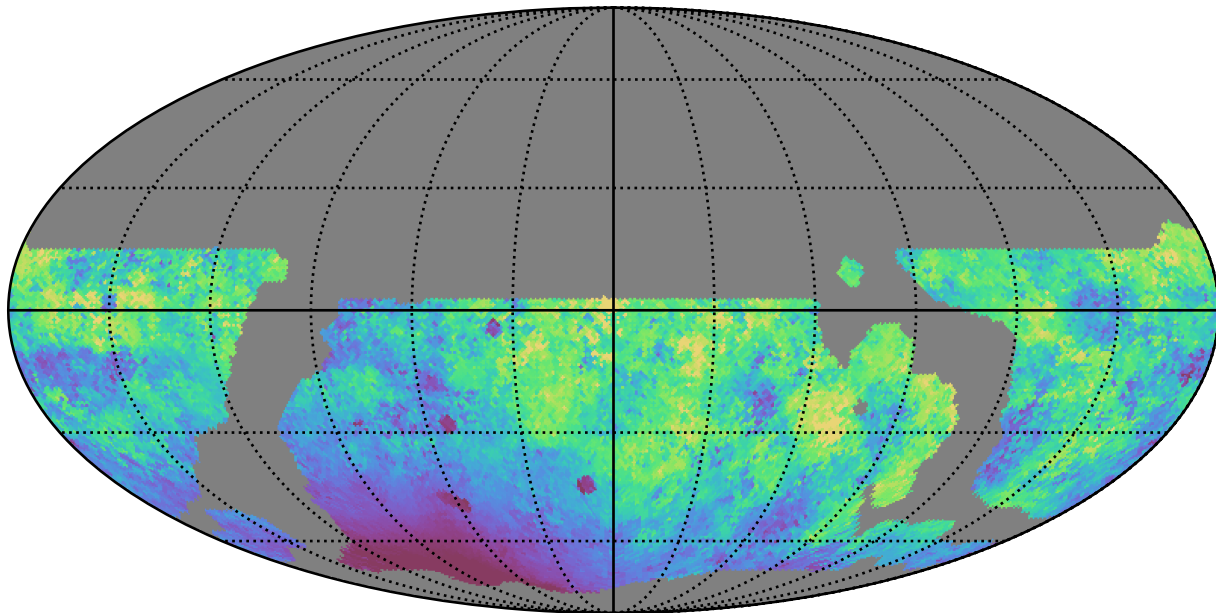
weather_cloudso6v3.4_10yrs WFD g band: Median moonDistance
