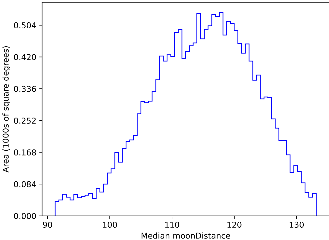
weather_cloudso6v3.4_10yrs WFD g band: Median moonDistance
