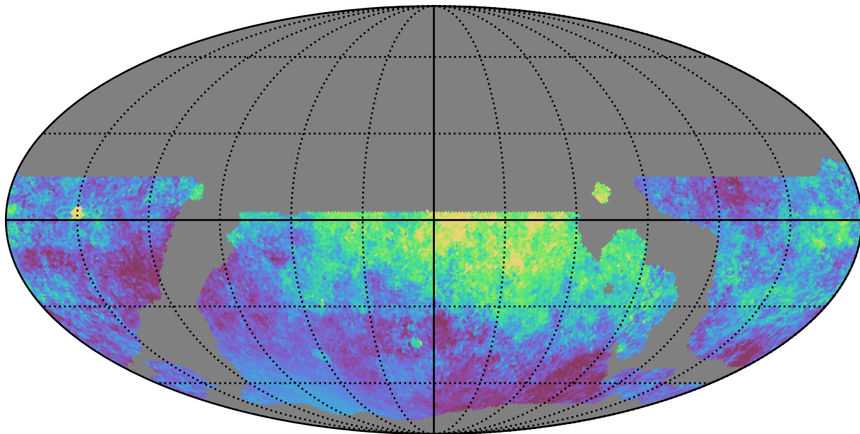
weather_cloudso6v3.4_10yrs WFD all bands: Median moonDistance
