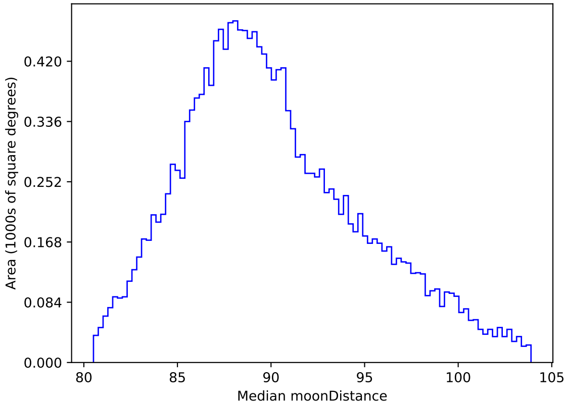
weather_cloudso6v3.4_10yrs WFD all bands: Median moonDistance
