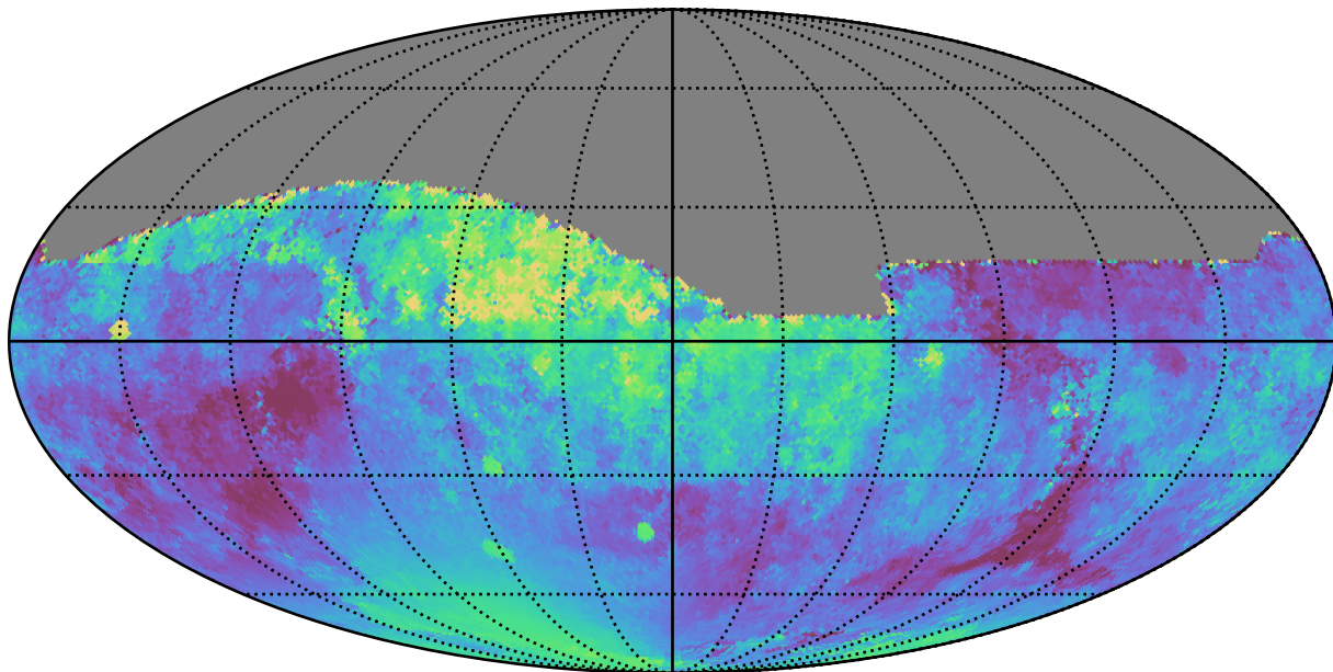
weather_cloudso6v3.4_10yrs All sky z band: Median moonDistance
