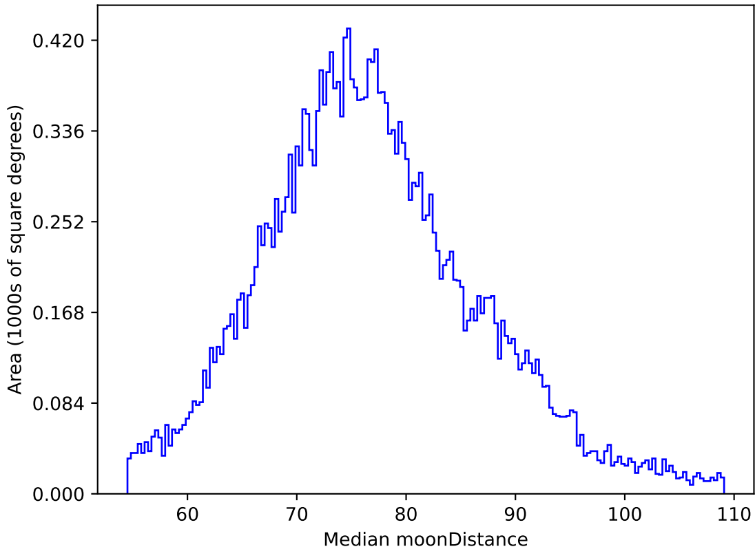
weather_cloudso6v3.4_10yrs All sky z band: Median moonDistance
