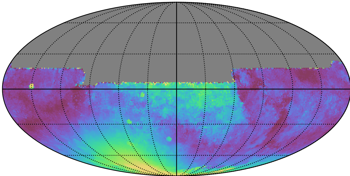
weather_cloudso6v3.4_10yrs All sky y band: Median moonDistance
