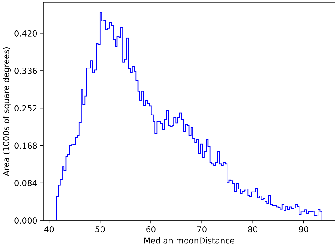
weather_cloudso6v3.4_10yrs All sky y band: Median moonDistance
