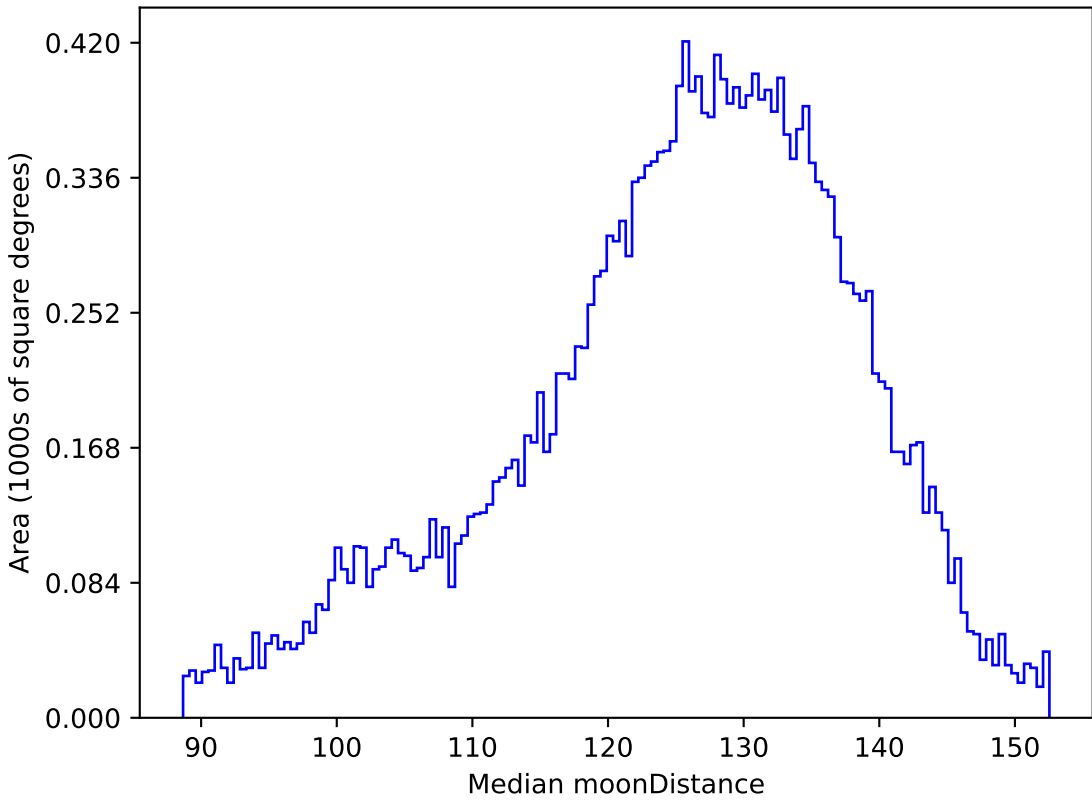
weather_cloudso6v3.4_10yrs All sky u band: Median moonDistance
