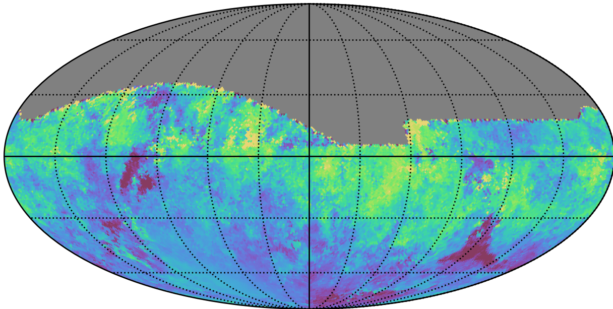
weather_cloudso6v3.4_10yrs All sky i band: Median moonDistance
