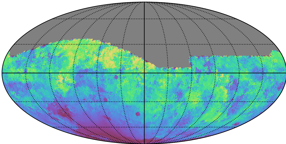
weather_cloudso6v3.4_10yrs All sky g band: Median moonDistance
