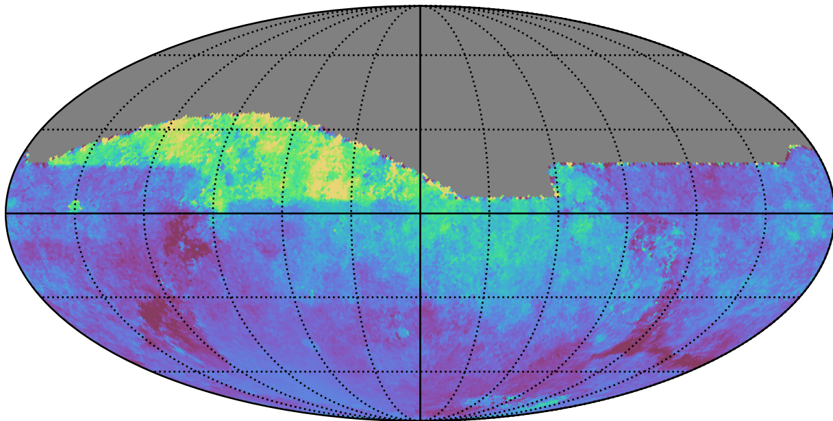
weather_cloudso6v3.4_10yrs All sky all bands: Median moonDistance
