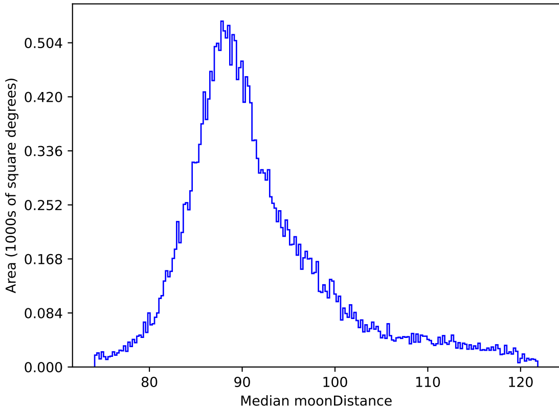
weather_cloudso6v3.4_10yrs All sky all bands: Median moonDistance
