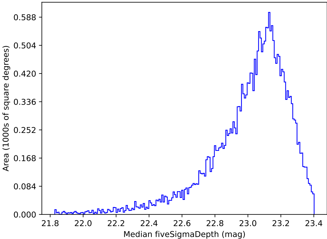
weather_cloudso6v3.4_10yrs Yr 1 z band: Median fiveSigmaDepth
