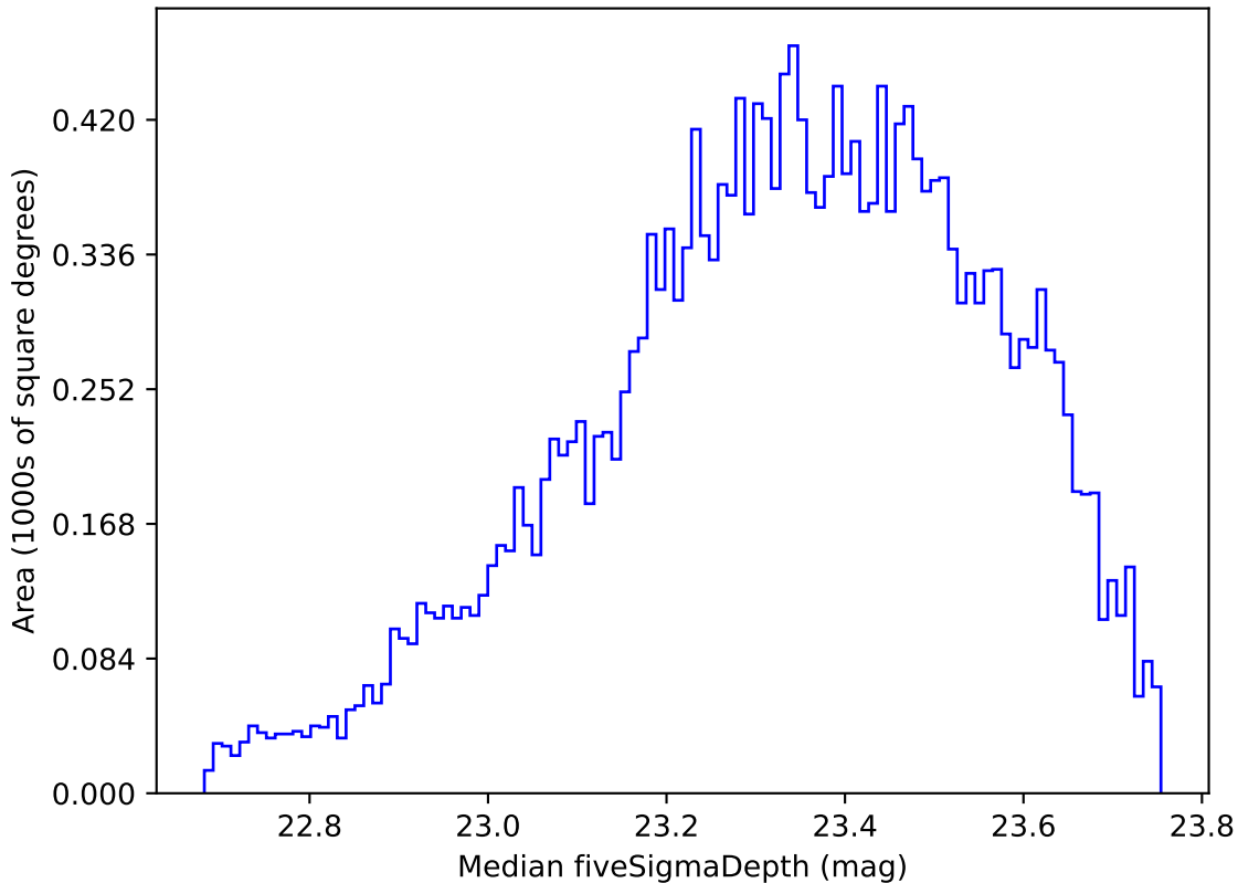
weather_cloudso6v3.4_10yrs Yr 1 u band: Median fiveSigmaDepth
