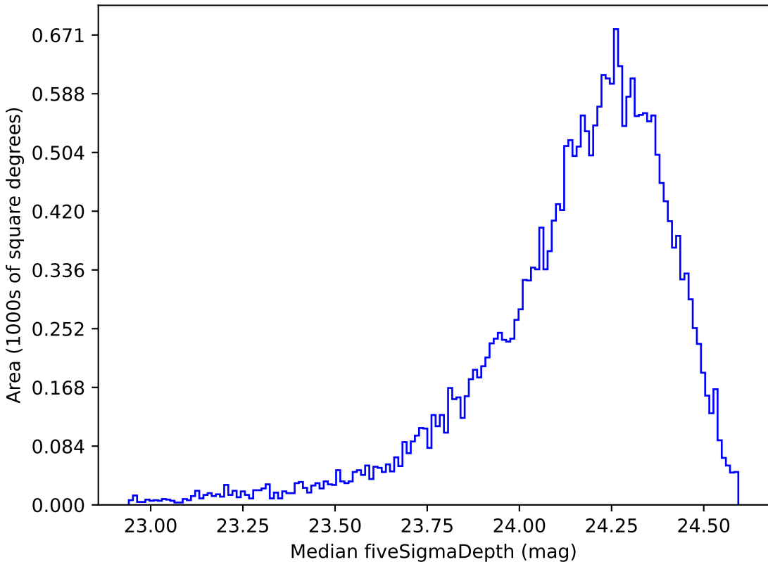
weather_cloudso6v3.4_10yrs Yr 1 r band: Median fiveSigmaDepth
