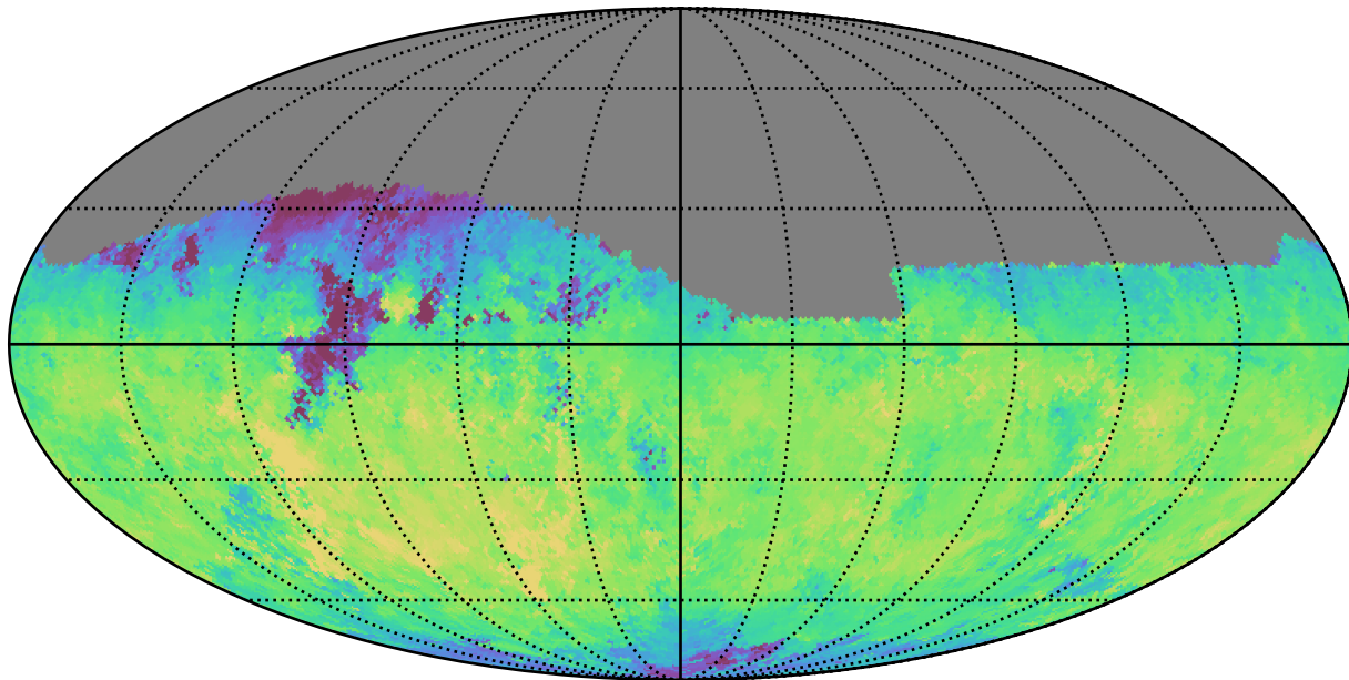
weather_cloudso6v3.4_10yrs Yr 1 i band: Median fiveSigmaDepth
