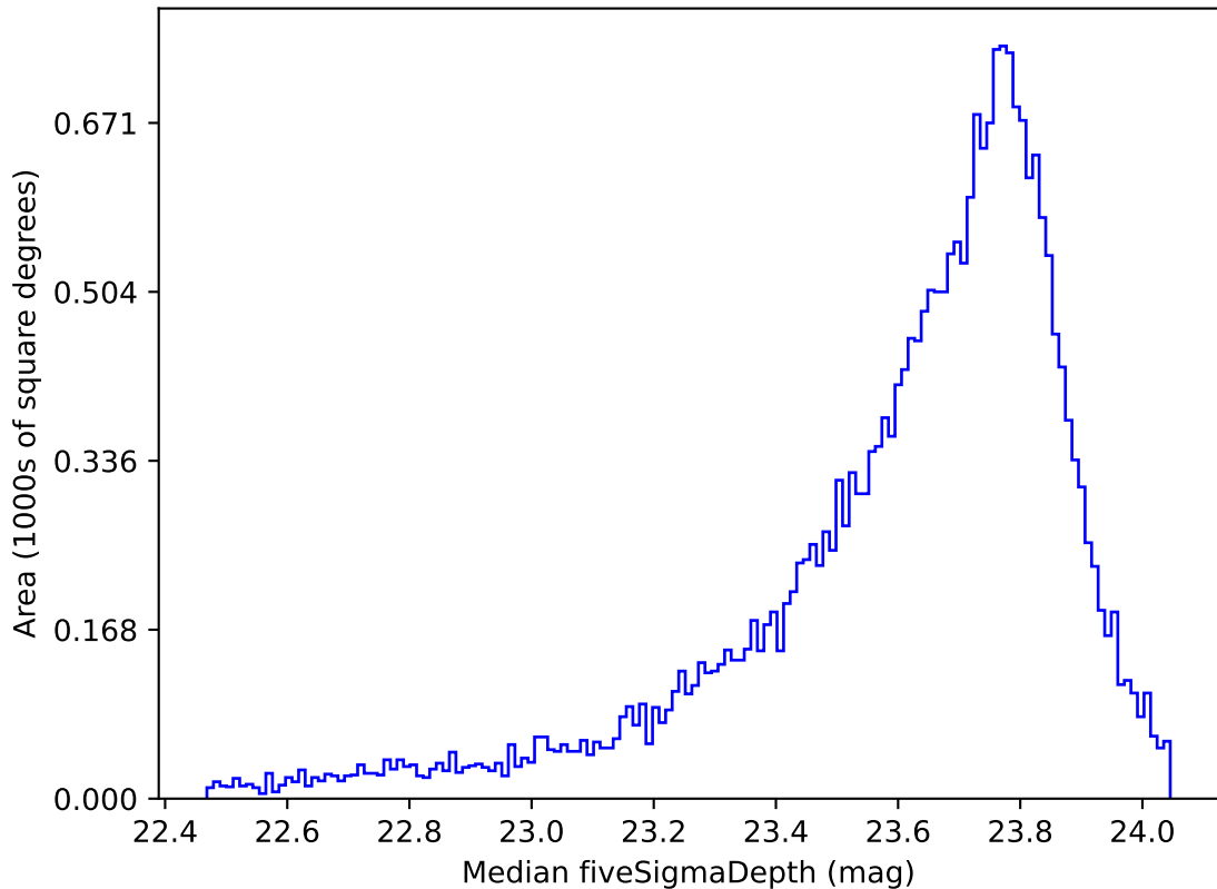
weather_cloudso6v3.4_10yrs Yr 1 i band: Median fiveSigmaDepth
