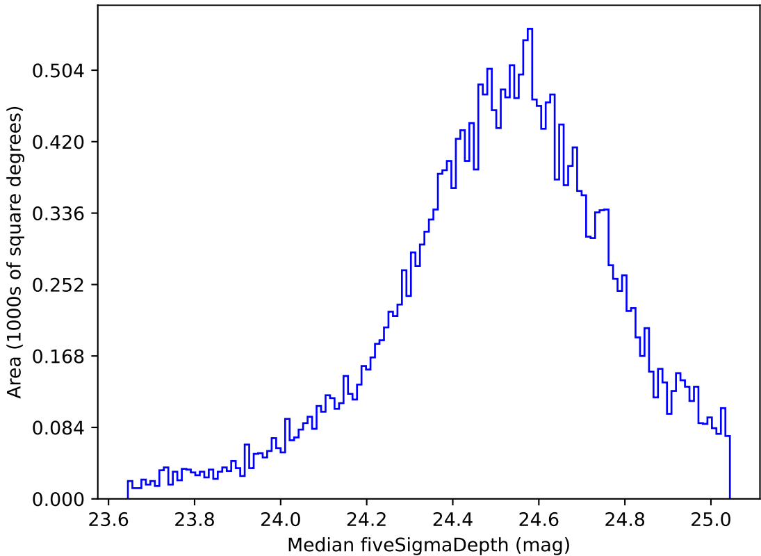
weather_cloudso6v3.4_10yrs Yr 1 g band: Median fiveSigmaDepth
