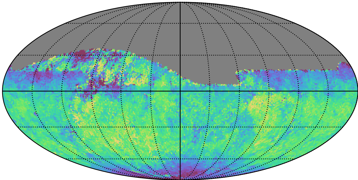
weather_cloudso6v3.4_10yrs Yr 1 all bands: Median fiveSigmaDepth
