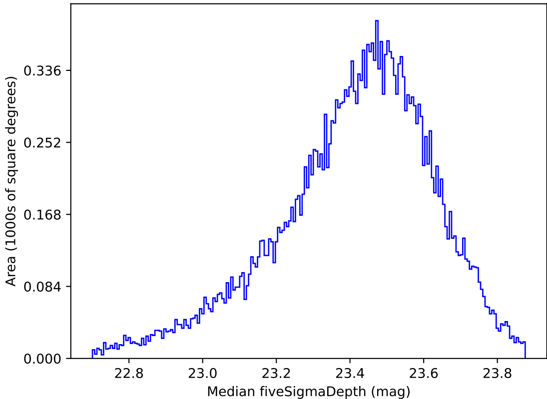
weather_cloudso6v3.4_10yrs Yr 1 all bands: Median fiveSigmaDepth
