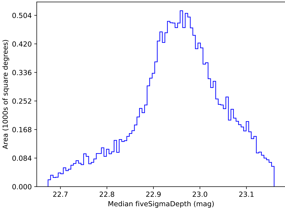
weather_cloudso6v3.4_10yrs WFD z band: Median fiveSigmaDepth
