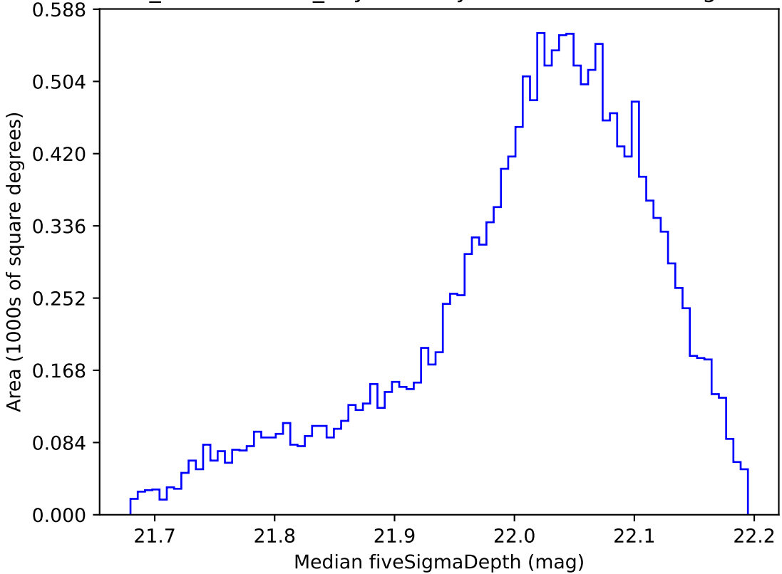
weather_cloudso6v3.4_10yrs WFD y band: Median fiveSigmaDepth
