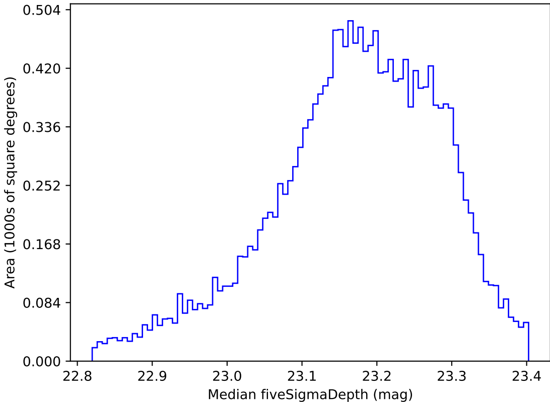
weather_cloudso6v3.4_10yrs WFD u band: Median fiveSigmaDepth
