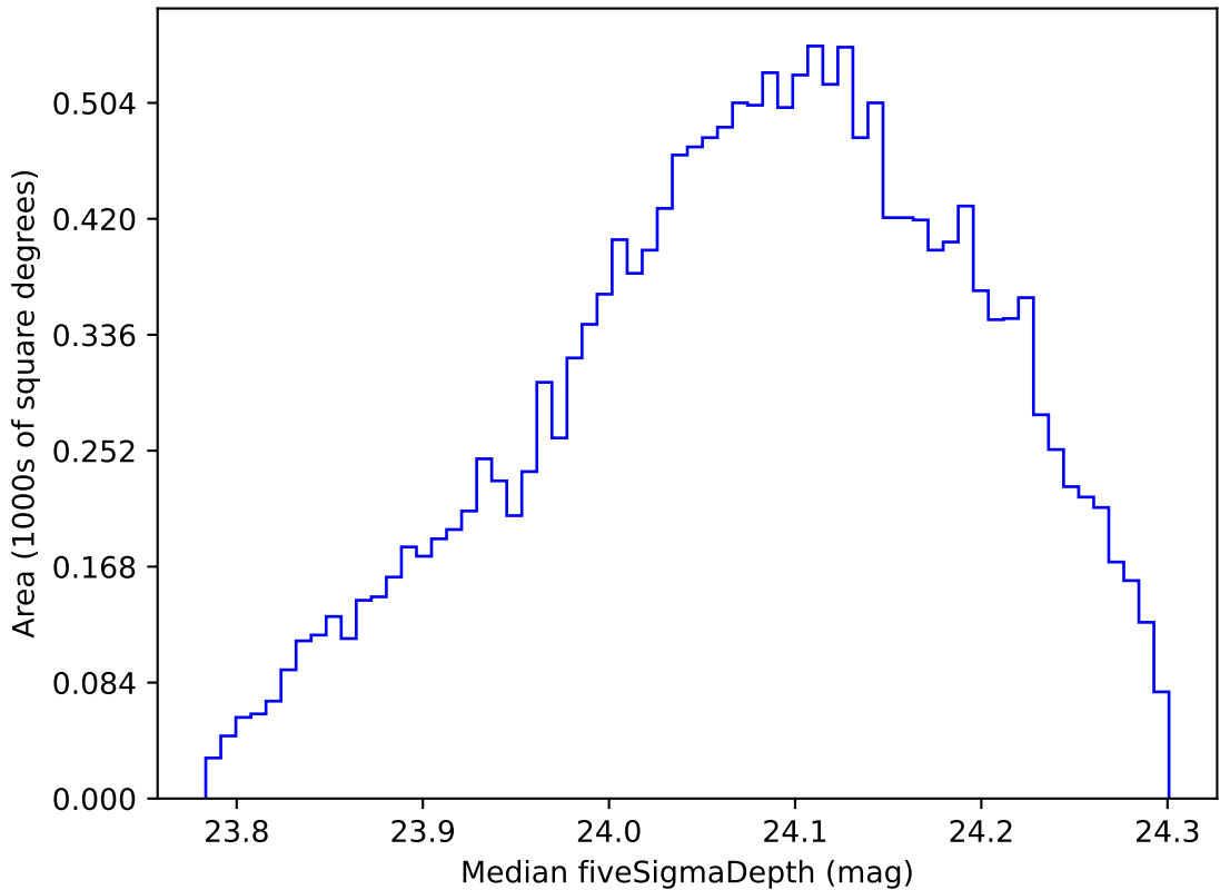
weather_cloudso6v3.4_10yrs WFD r band: Median fiveSigmaDepth
