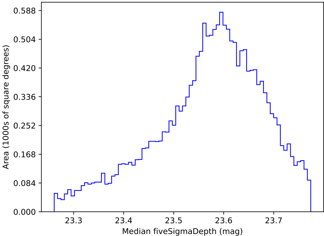
weather_cloudso6v3.4_10yrs WFD i band: Median fiveSigmaDepth
