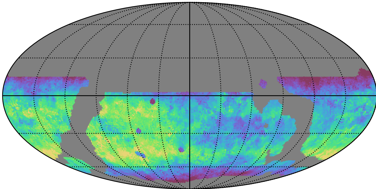
weather_cloudso6v3.4_10yrs WFD g band: Median fiveSigmaDepth
