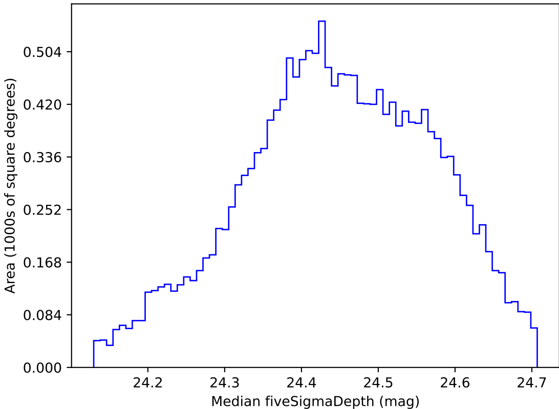
weather_cloudso6v3.4_10yrs WFD g band: Median fiveSigmaDepth
