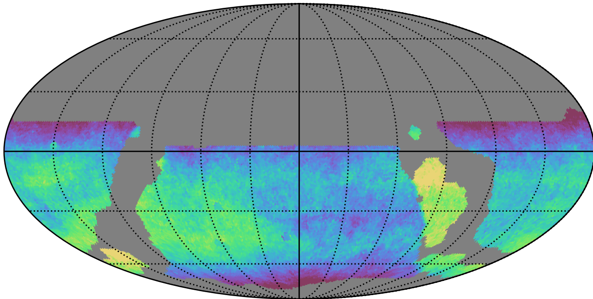
weather_cloudso6v3.4_10yrs WFD all bands: Median fiveSigmaDepth
