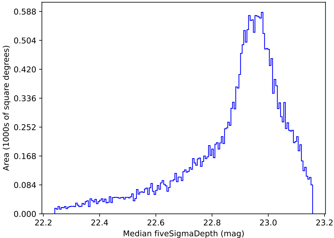
weather_cloudso6v3.4_10yrs All sky z band: Median fiveSigmaDepth
