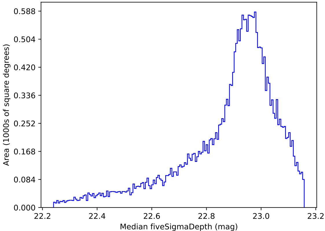
weather_cloudso6v3.4_10yrs All sky z band: Median fiveSigmaDepth
