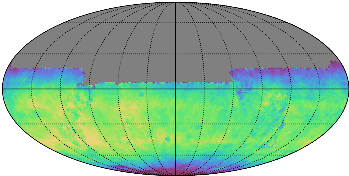
weather_cloudso6v3.4_10yrs All sky y band: Median fiveSigmaDepth
