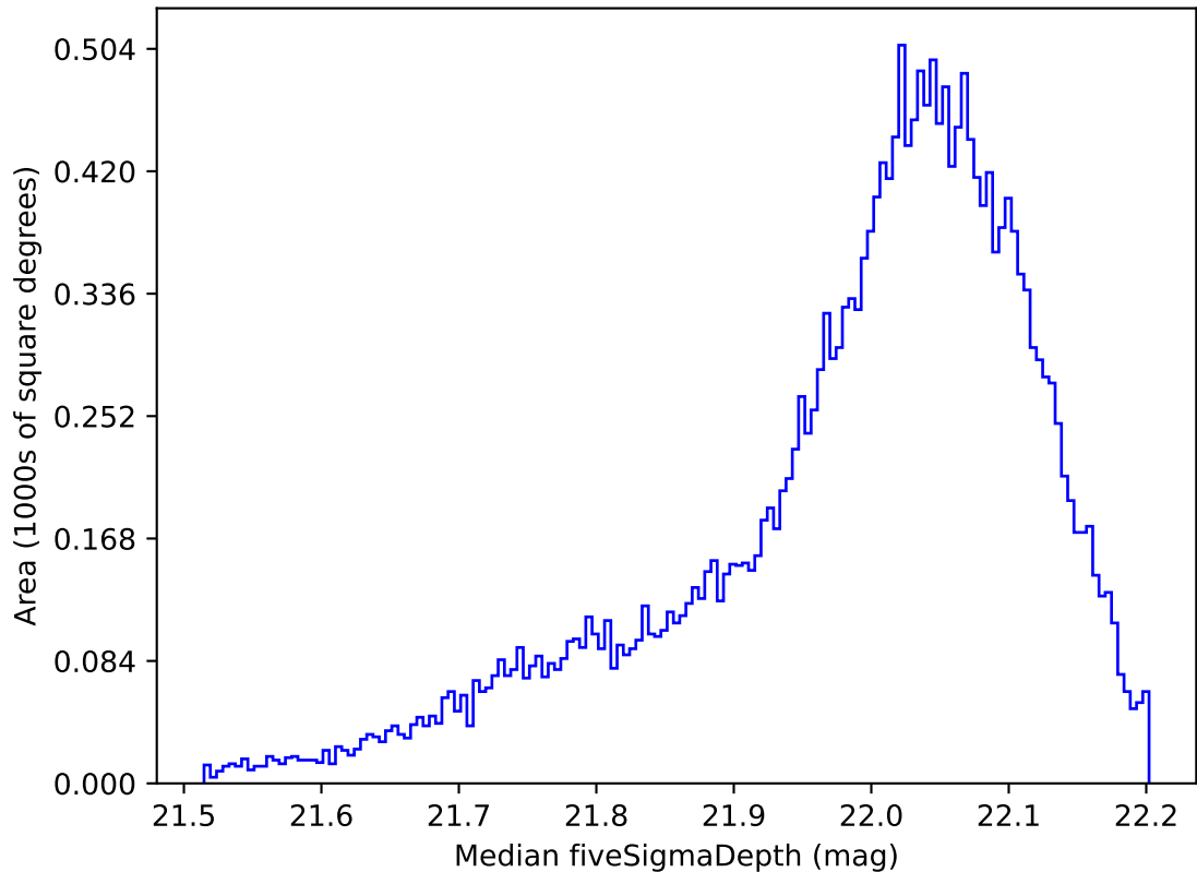
weather_cloudso6v3.4_10yrs All sky y band: Median fiveSigmaDepth
