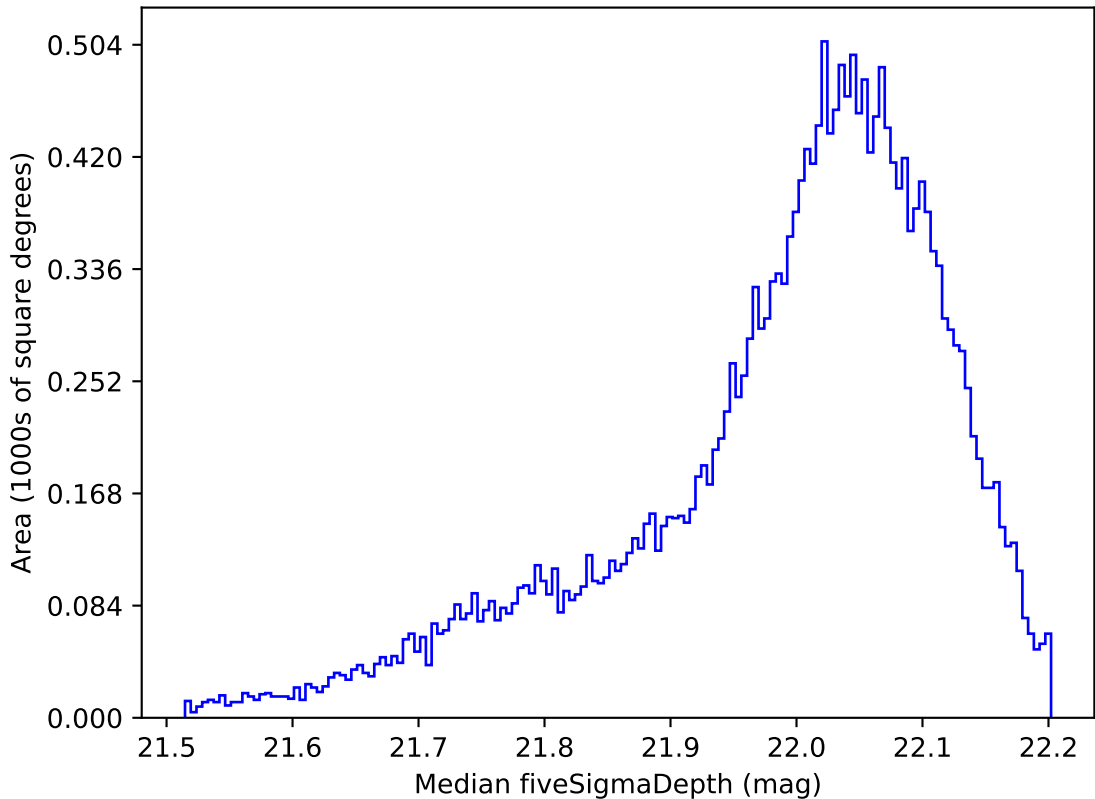
weather_cloudso6v3.4_10yrs All sky y band: Median fiveSigmaDepth
