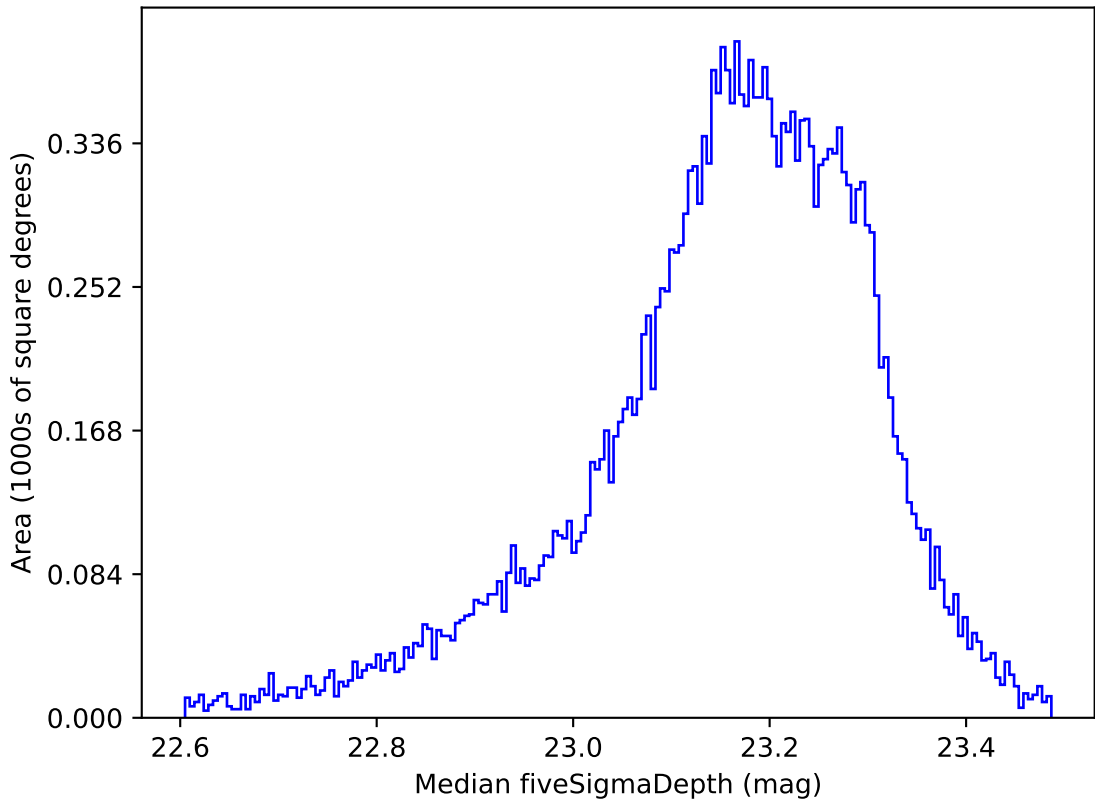
weather_cloudso6v3.4_10yrs All sky u band: Median fiveSigmaDepth
