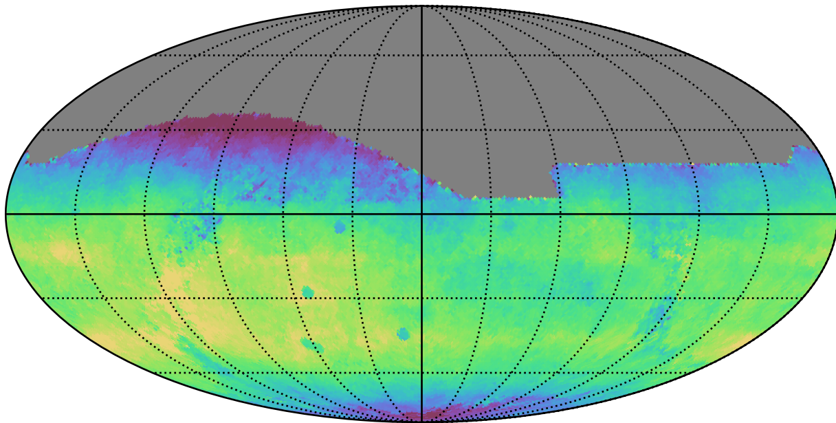
weather_cloudso6v3.4_10yrs All sky r band: Median fiveSigmaDepth
