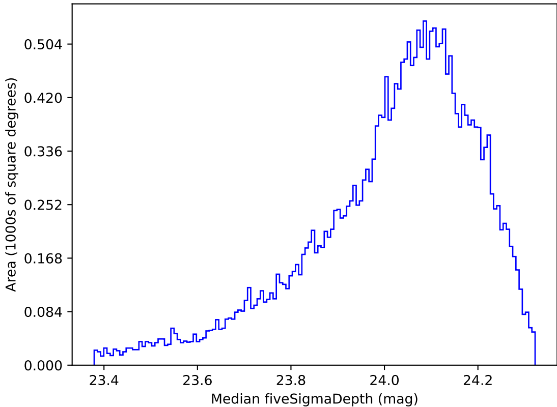
weather_cloudso6v3.4_10yrs All sky r band: Median fiveSigmaDepth
