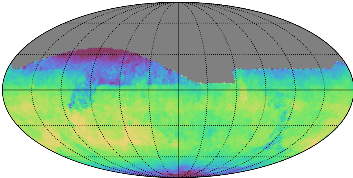
weather_cloudso6v3.4_10yrs All sky i band: Median fiveSigmaDepth
