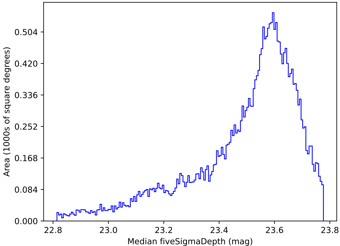
weather_cloudso6v3.4_10yrs All sky i band: Median fiveSigmaDepth
