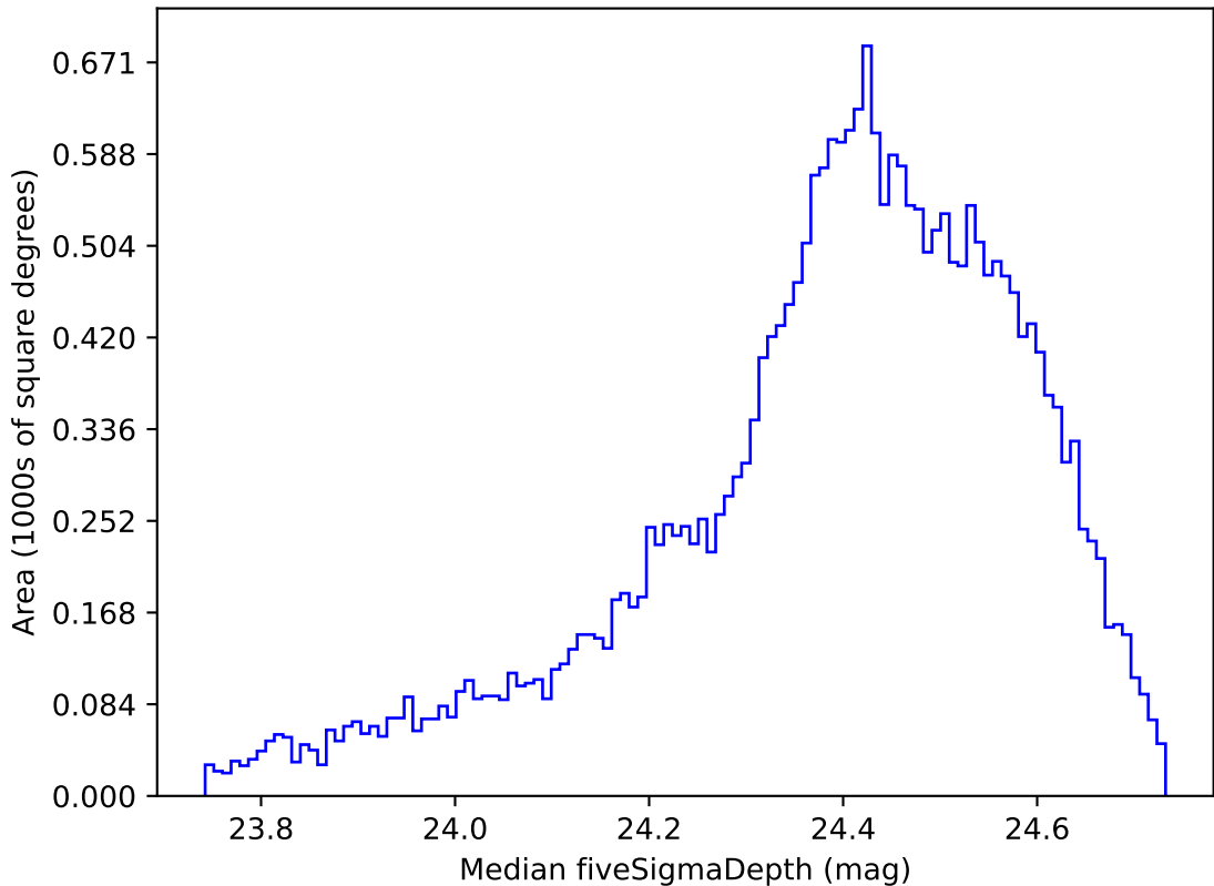
weather_cloudso6v3.4_10yrs All sky g band: Median fiveSigmaDepth
