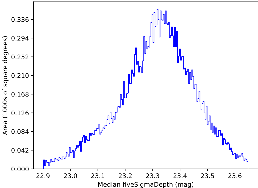
weather_cloudso6v3.4_10yrs All sky all bands: Median fiveSigmaDepth
