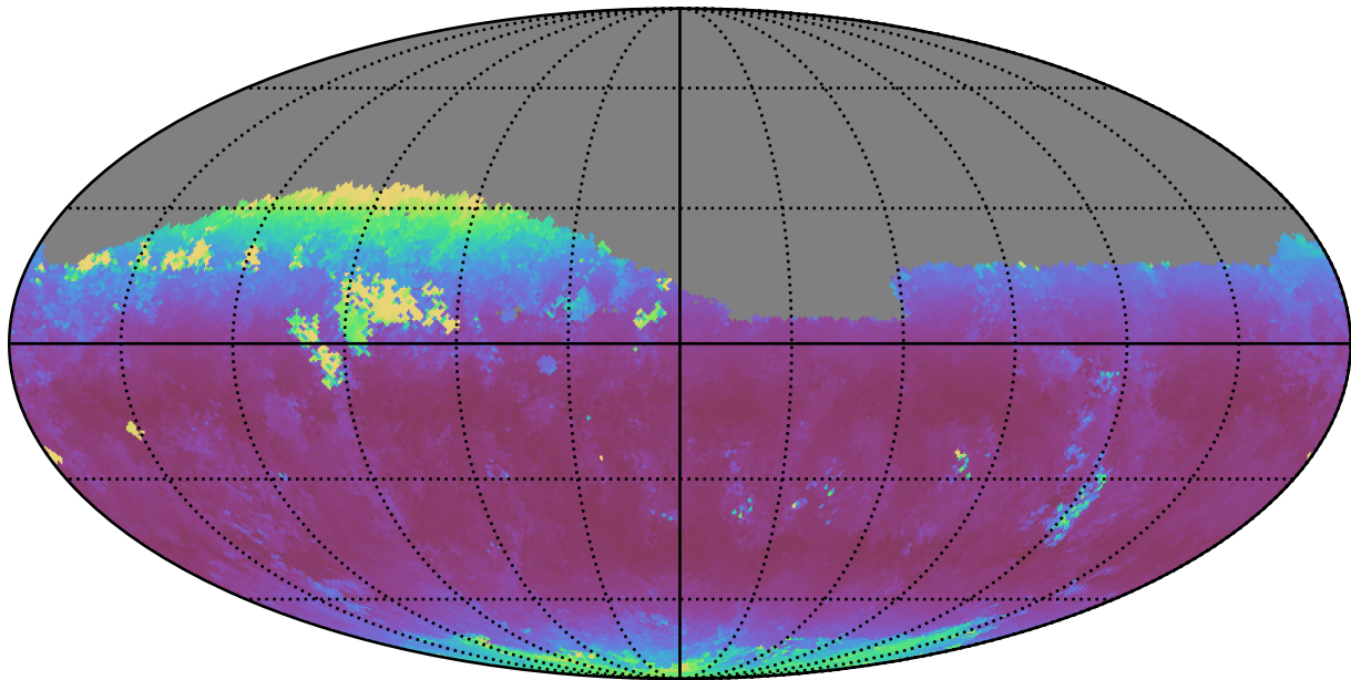
weather_cloudso6v3.4_10yrs Yr 1 z band: Median airmass
