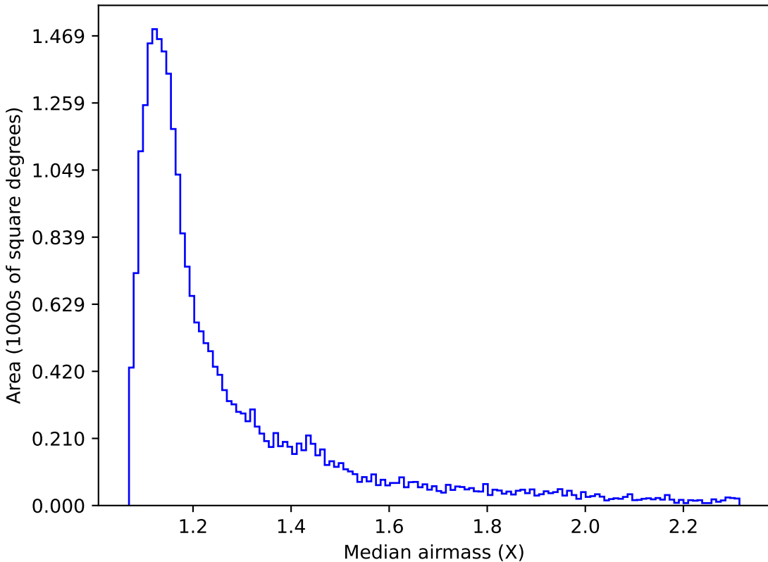
weather_cloudso6v3.4_10yrs Yr 1 z band: Median airmass
