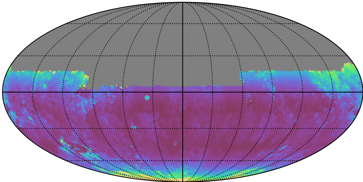
weather_cloudso6v3.4_10yrs Yr 1 y band: Median airmass
