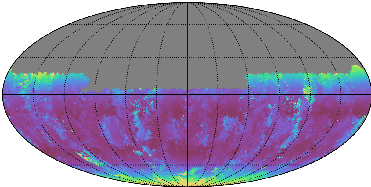
weather_cloudso6v3.4_10yrs Yr 1 u band: Median airmass
