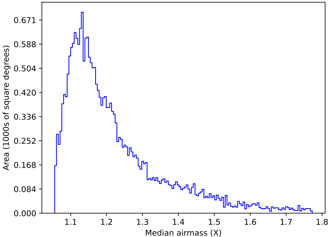
weather_cloudso6v3.4_10yrs Yr 1 u band: Median airmass
