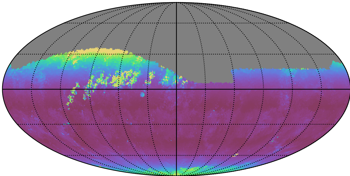
weather_cloudso6v3.4_10yrs Yr 1 r band: Median airmass
