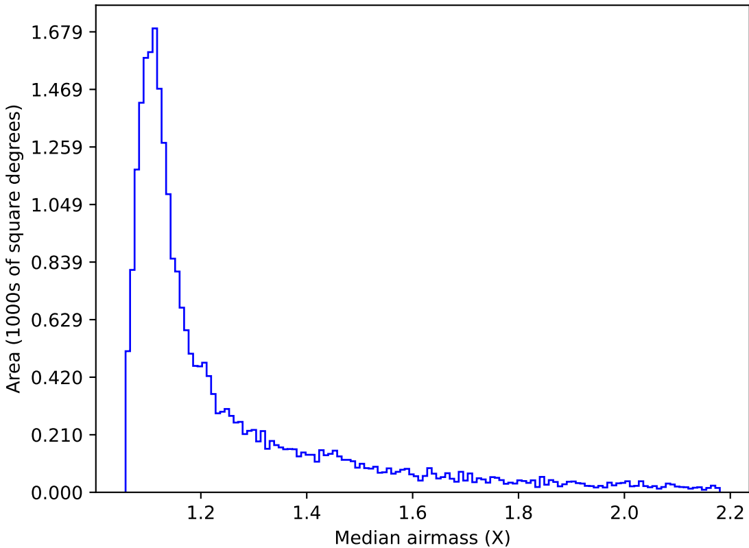
weather_cloudso6v3.4_10yrs Yr 1 r band: Median airmass
