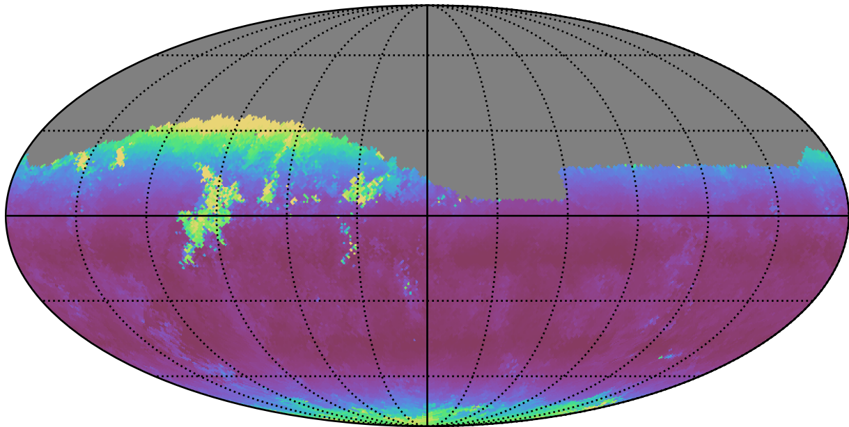
weather_cloudso6v3.4_10yrs Yr 1 i band: Median airmass
